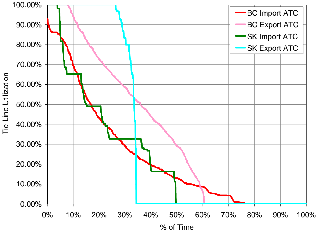
Figure 10 - Tie Line Utilization (Q1/07)
